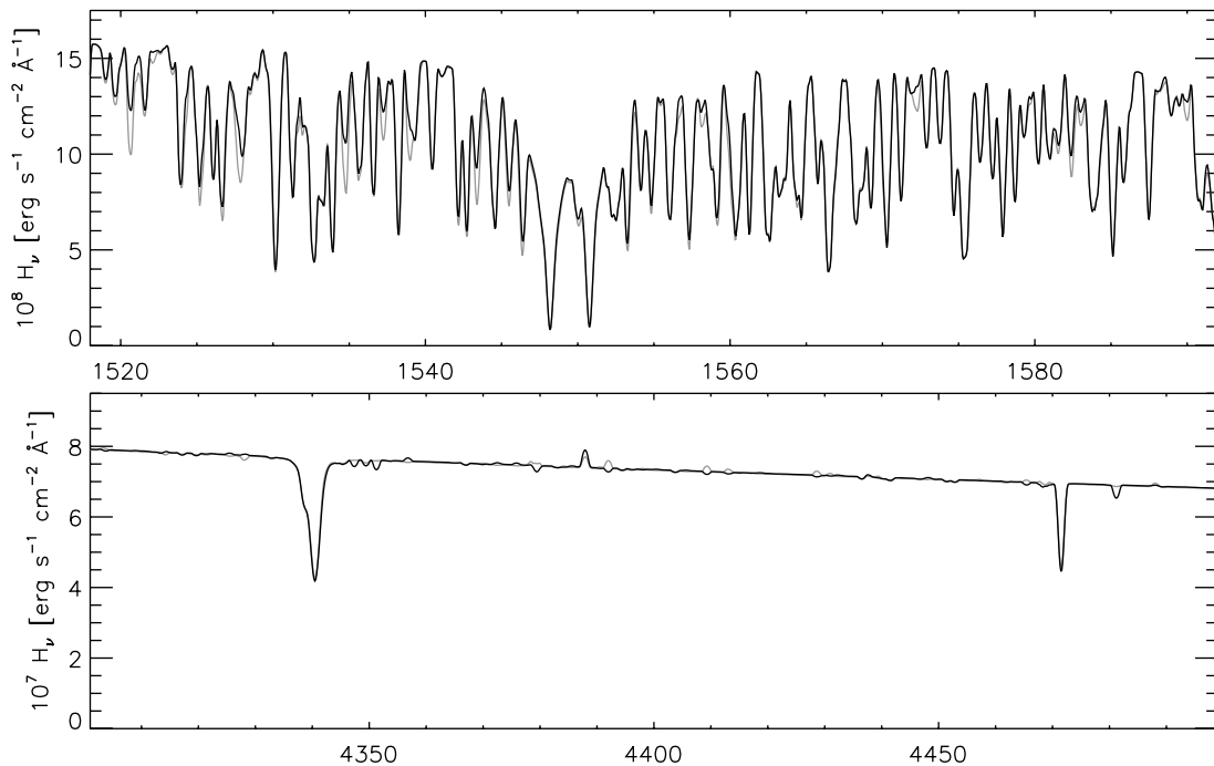
FIG. 4.—Ultraviolet and visible model spectra for model atmospheres with identical stellar parameters ( T_{\text{eff}} = 30,000 K, \log g = 3.0 , solar composition, and V_i = 10 km \text{s}^{-1} ) from the two grids: BSTAR2006 (black line) and OSTAR2002 (gray line). A rotational broadening of 50 km \text{s}^{-1} was applied to the spectra. [See the electronic edition of the Supplement for a color version of this figure.]
