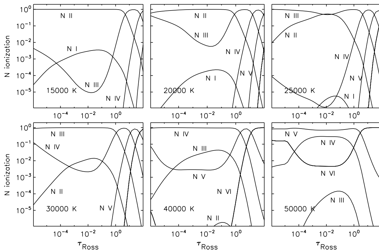
FIG. 10.—Ionization fractions of nitrogen as function of depth in six NLTE model atmospheres, T_{\text{eff}} = 15,000, 20,000, 25,000, 30,000, 40,000, and 50,000 K, \log g = 4.0 , and solar composition. [See the electronic edition of the Supplement for a color version of this figure.]
