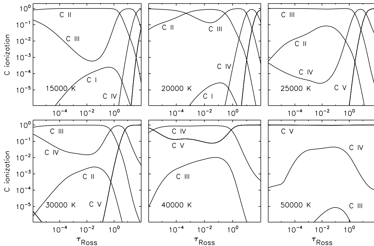
FIG. 9.—Ionization fractions of carbon as function of depth in six NLTE model atmospheres, T_{\text{eff}} = 15,000, 20,000, 25,000, 30,000, 40,000, and 50,000 K, \log g = 4.0 , and solar composition. [See the electronic edition of the Supplement for a color version of this figure.]
