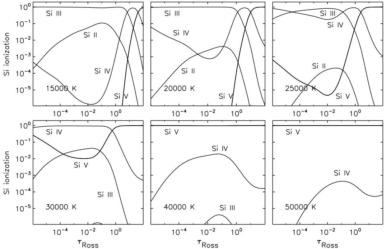
FIG. 14.—Ionization fractions of silicon as function of depth in six NLTE model atmospheres, T_{\text{eff}} = 15,000, 20,000, 25,000, 30,000, 40,000, and 50,000 K, \log g = 4.0 , and solar composition. [See the electronic edition of the Supplement for a color version of this figure.]
