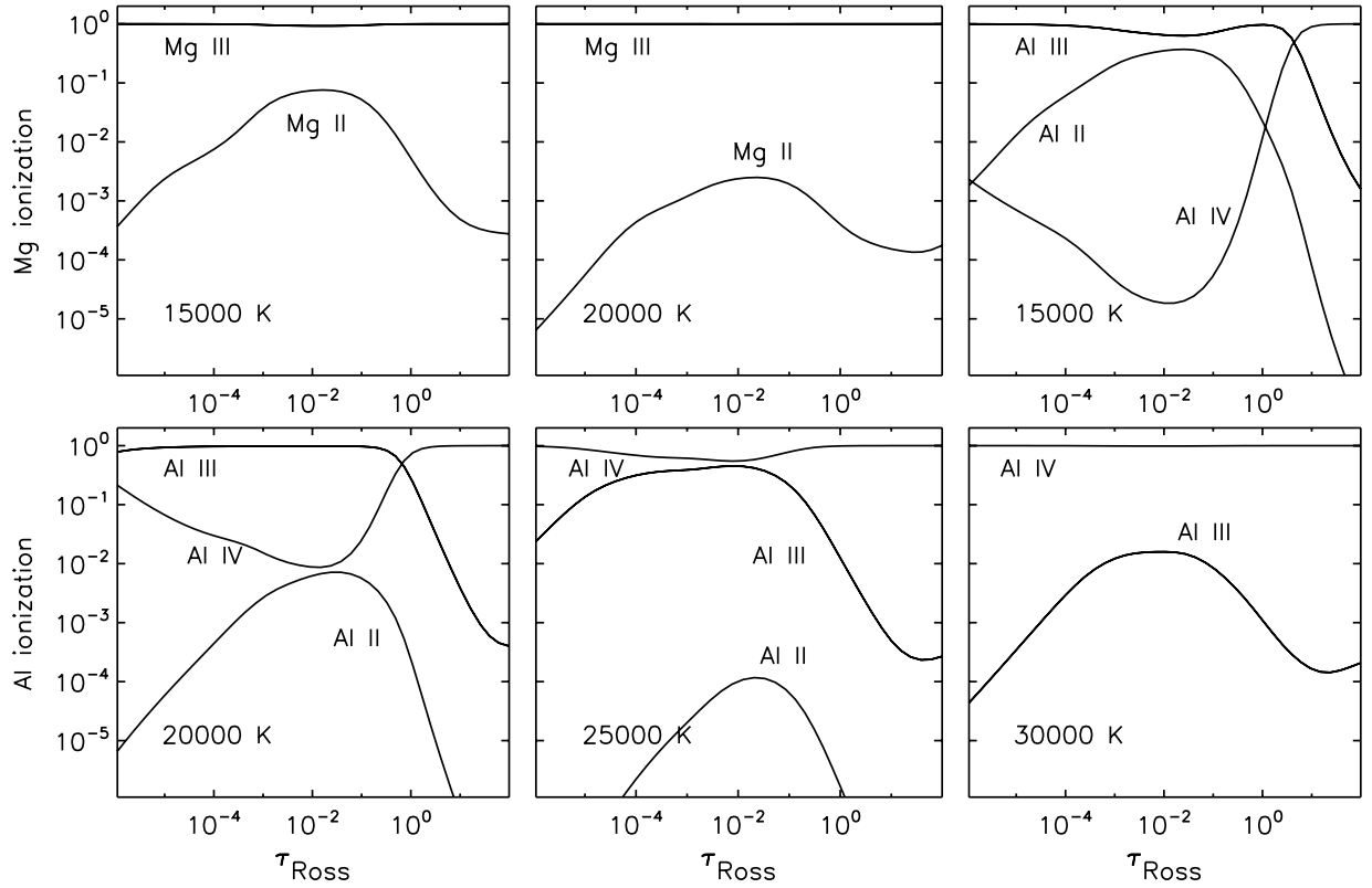
FIG. 13.—Ionization fractions of magnesium and aluminum as function of depth in four NLTE model atmospheres, T_{\text{eff}} = 15,000, 20,000, 25,000, and 30,000 K, \log g = 4.0 , and solar composition. [See the electronic edition of the Supplement for a color version of this figure.]
