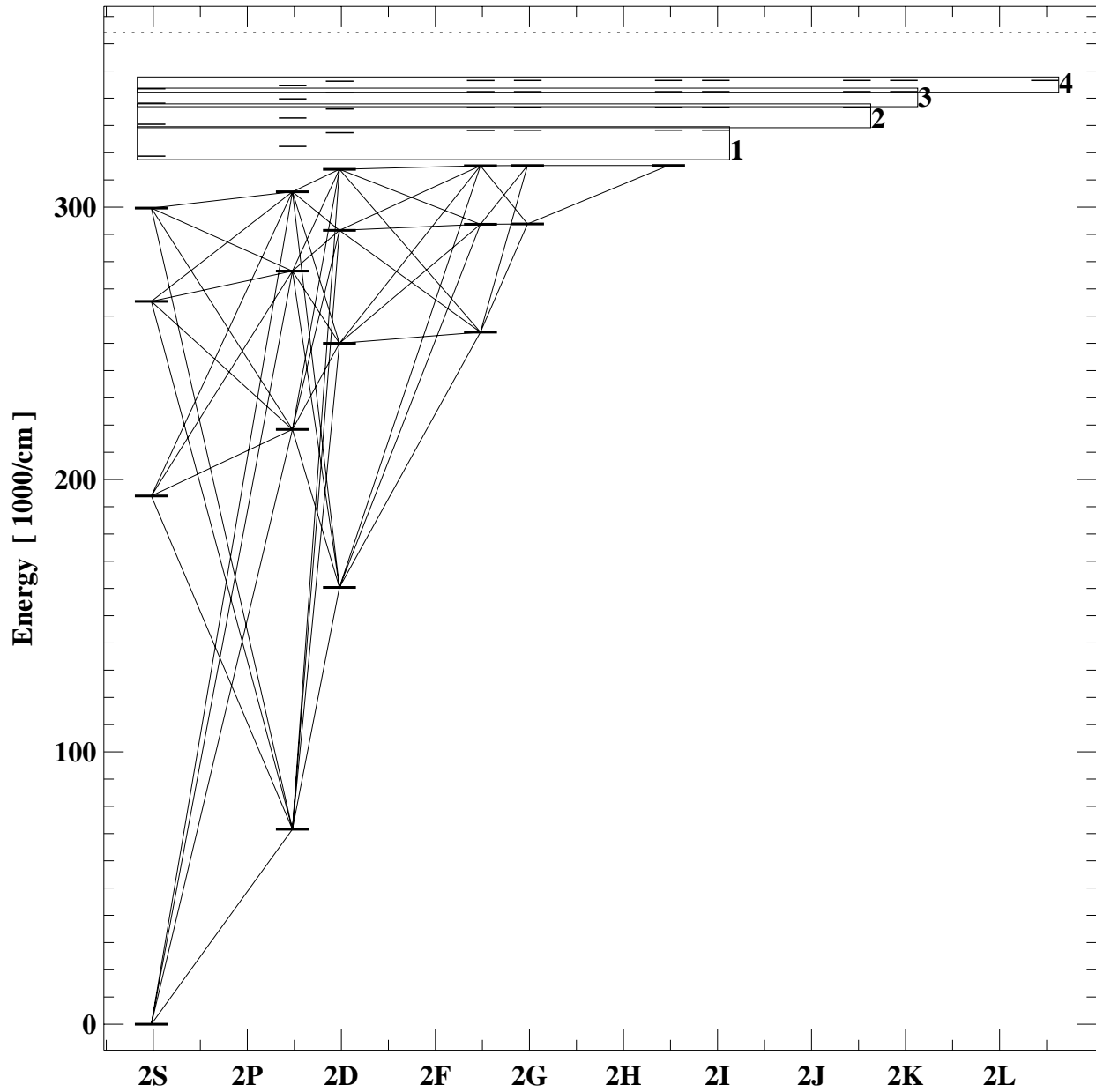
Grotrian diagram for si4
