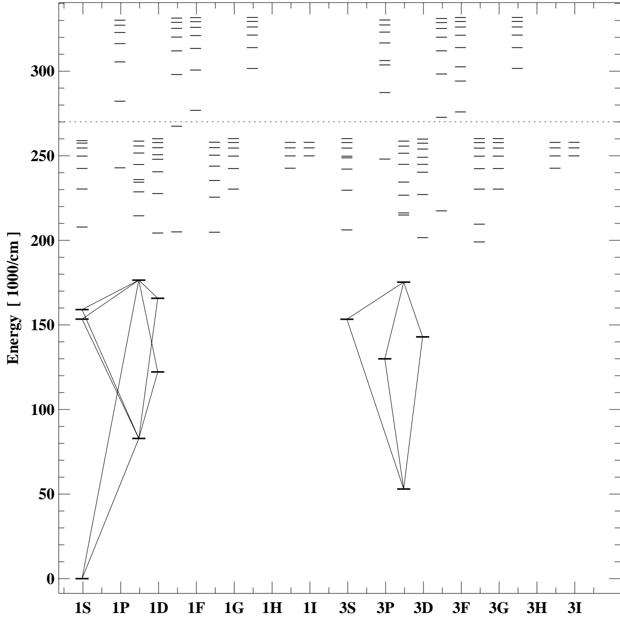
Grotrian diagram for si3
