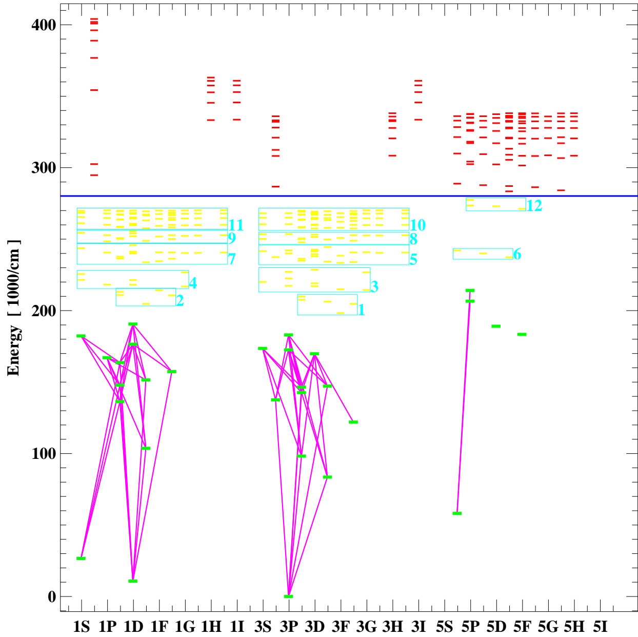
Grotrian diagram for s3
