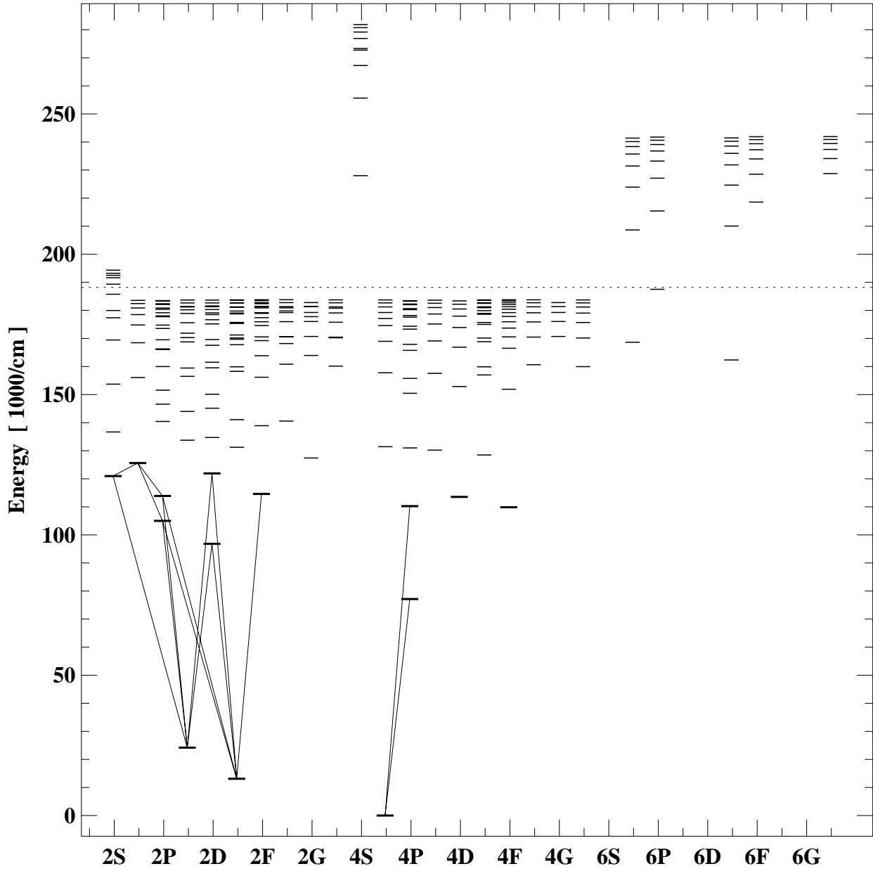
Grotrian diagram for s2
