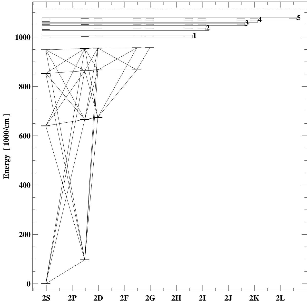
Grotrian diagram for o6
