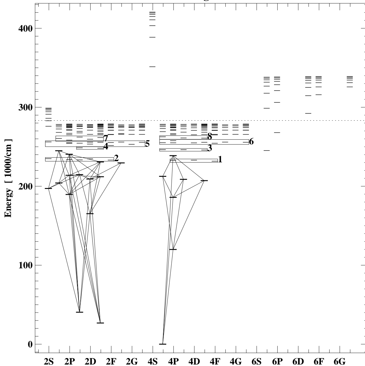
Grotrian diagram for o2
