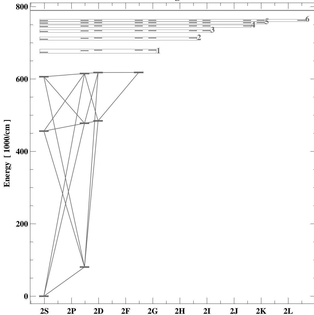
Grotrian diagram for n5
