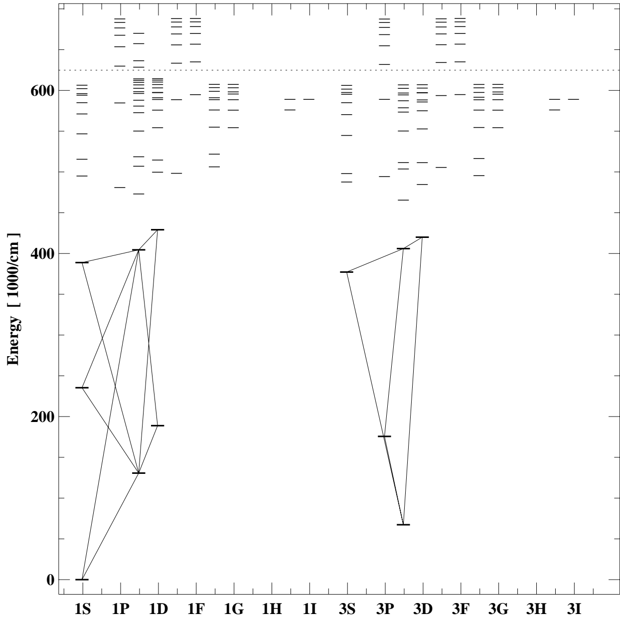
Grotrian diagram for n4
