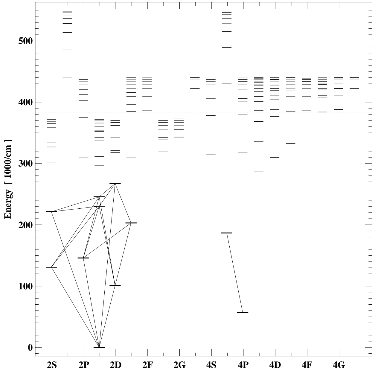
Grotrian diagram for n3
