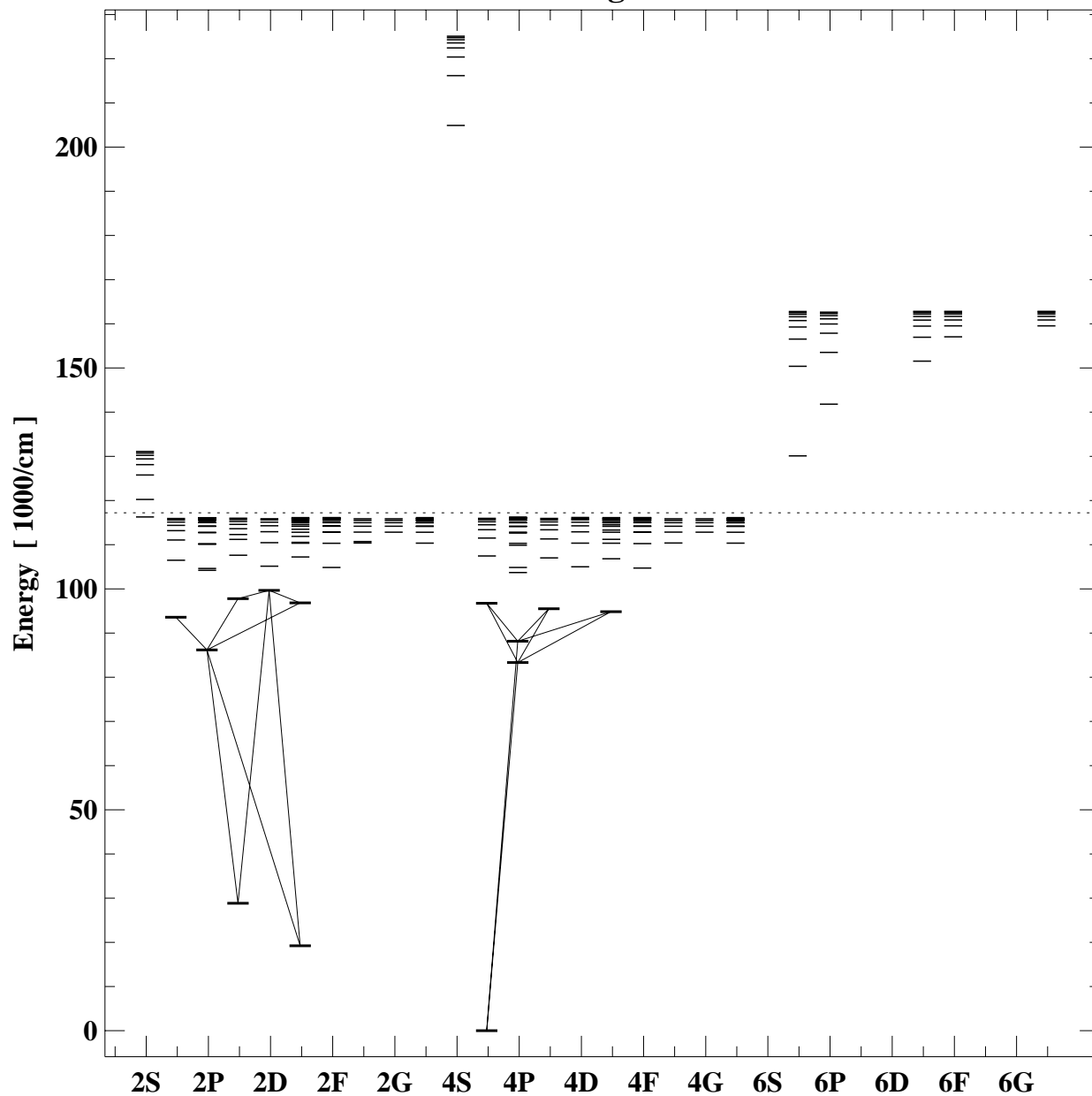
Grotrian diagram for n1
