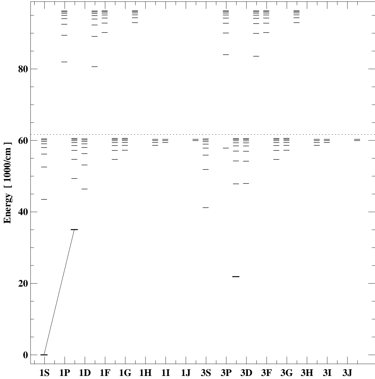
Grotrian diagram for mg1
