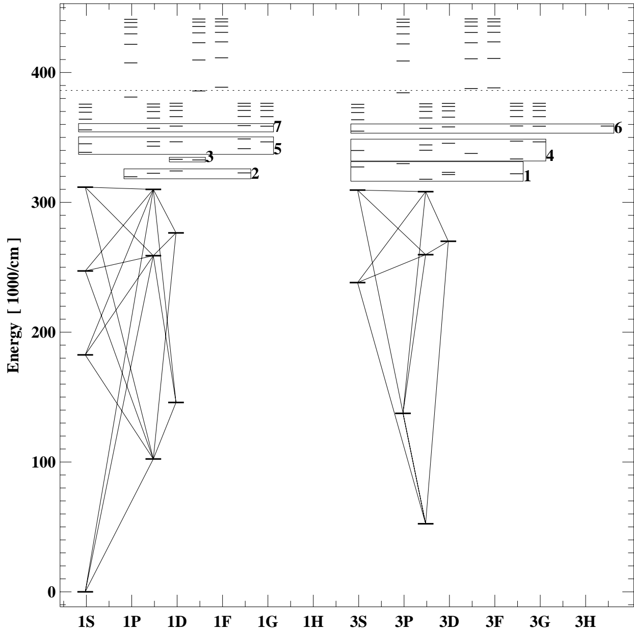
Grotrian diagram for c3
