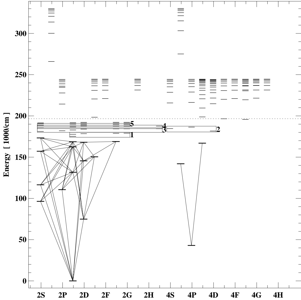
Grotrian diagram for c2
